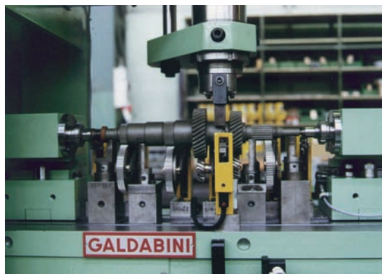
Automatic straightening machine 50 tons - Output gearbox shaft - Final runout 30 microns
